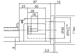
Motor Adaptor Flange F5
