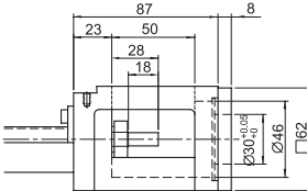
Motor Adaptor Flange F3
