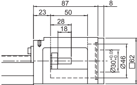
Motor Adaptor Flange F2
