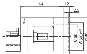
Motor Adaptor Flange F4
