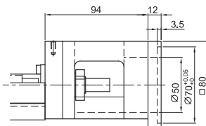
Motor Adaptor Flange F2
