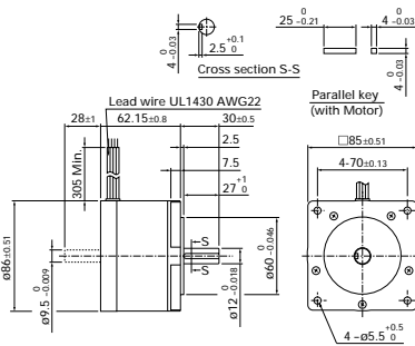
103H8581-7041/8041 (Single shaft) 103H8581-7011/8011 (Double shaft)
