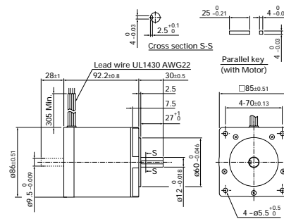
103H8582-7041/8041 (Single shaft) 103H8582-7011/8011 (Double shaft)
