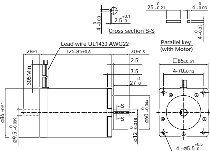
103H8583-7041/8041 (Single shaft) 103H8583-7011/8011 (Double shaft)
